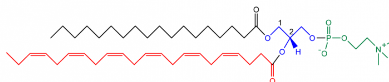
Phosphatidyl-choline with DHA and a second fatty acid (here stearic acid)
